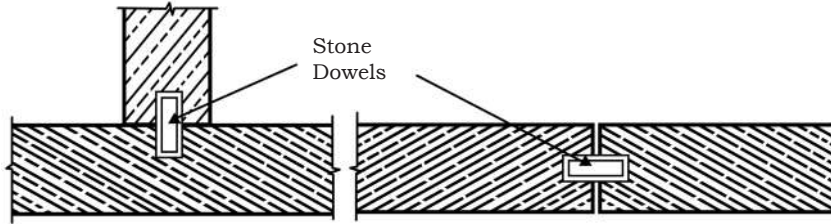
Fig. 1.25: Dowel Joint
