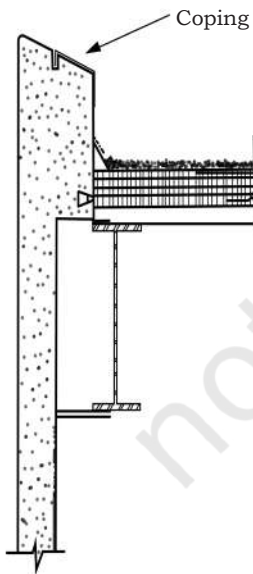
Fig. 1.3: Coping
