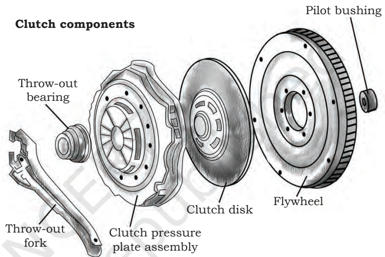
Fig. 3.24: Clutch assembly
