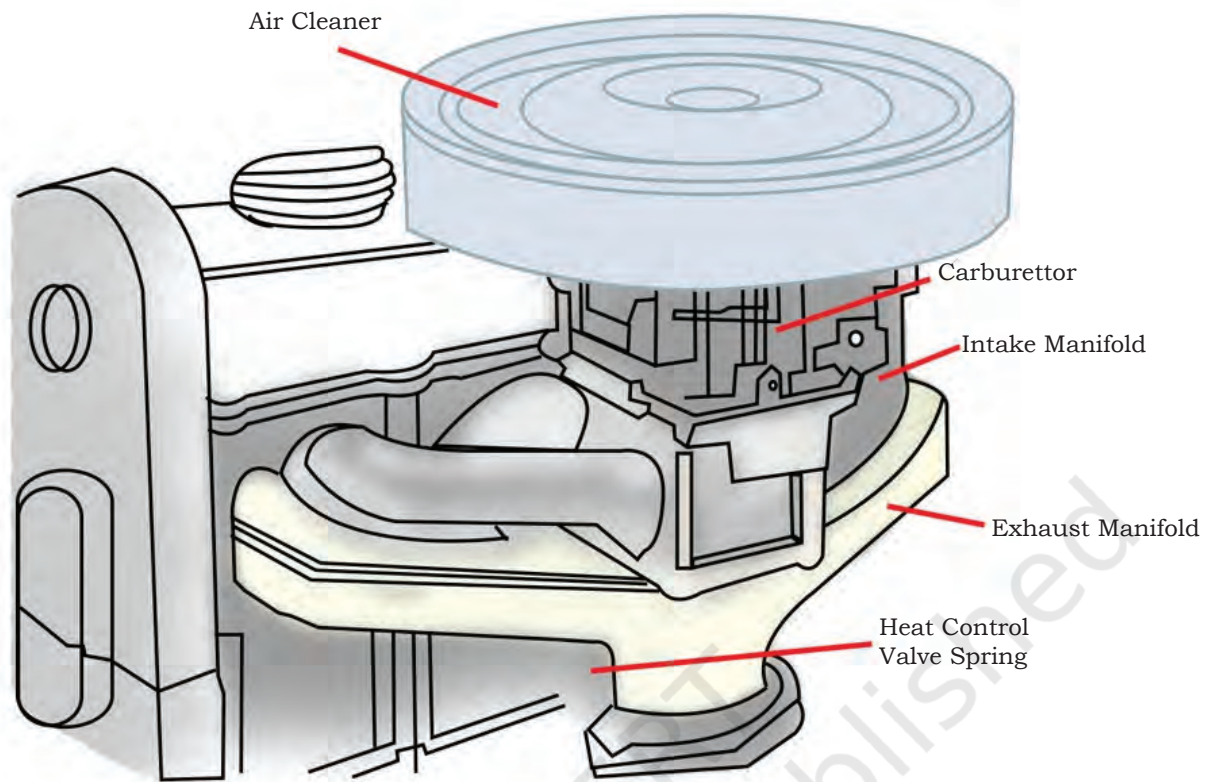
Fig. 3.8: Exhaust Manifold
